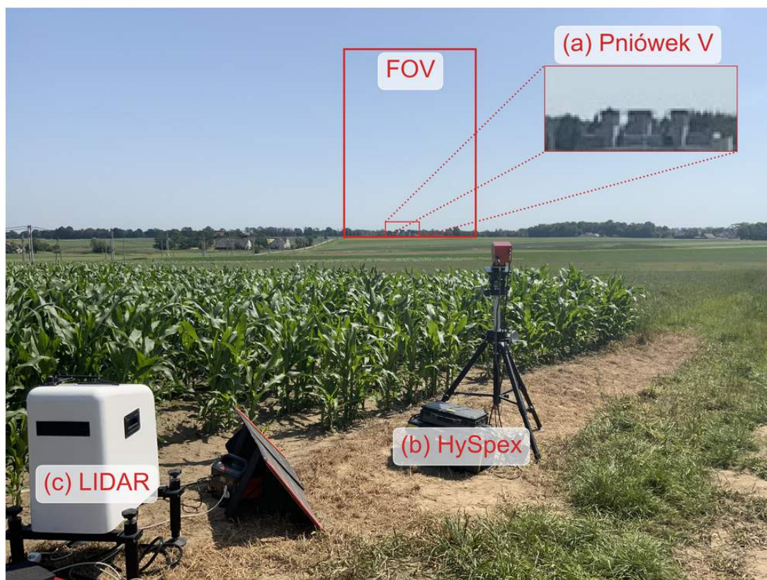
Figure 1: The instrumental setup. The inset shows the three ventilators of the coal mine shaft (a). The HySpex SWIR-284 camera (b) and the wind-lidar (c) are deployed at 1 km distance, the red rectangle shows the camera field of view (FOV).
