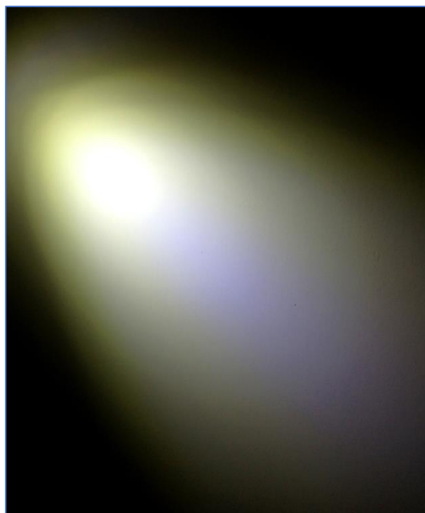
Figure 10: Phosphor white LED colour zoning – note the high CCT (blue tint) in the centre of the beam, surrounded by a yellow-tinted annulus.
