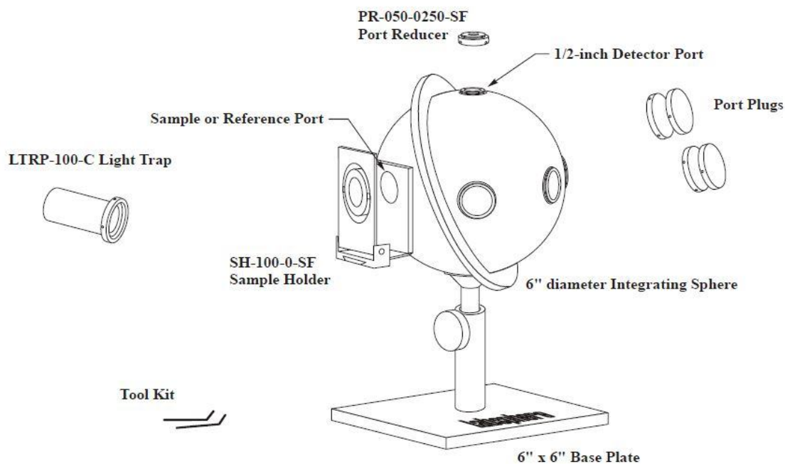
Figure 1: Standard attachments to the RT-060-SF. The port reducer, sample holders and port plugs accompanying the RT-060-IG sphere assembly are coated with Infragold.
