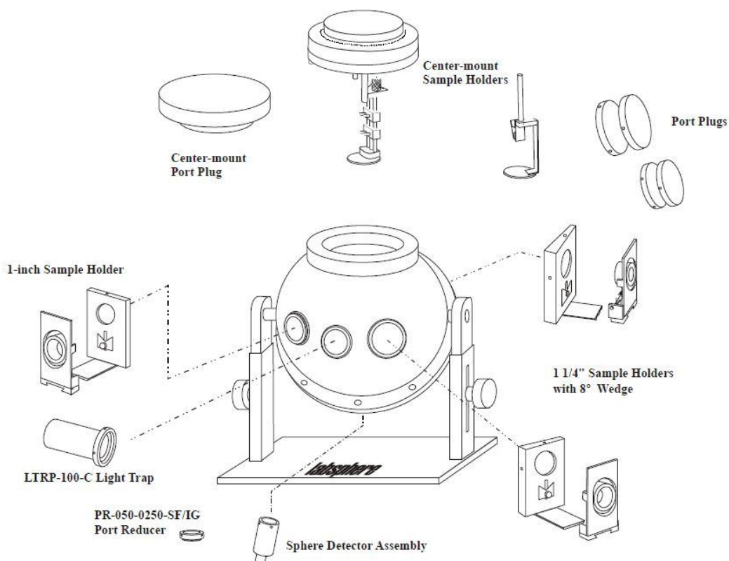
Figure 2: Standard attachments to the RTC series sphere assemblies.
